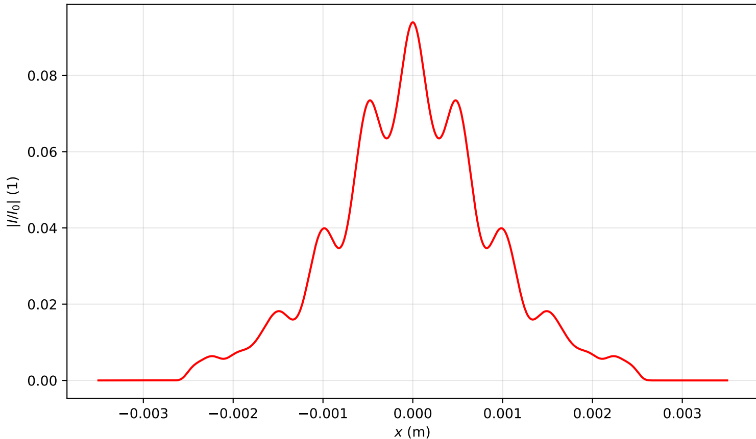
Intensity profile I(x, y = 0, z = 3.344)/I_0 , P_{in}=2.0P_{cr} , artificial time
